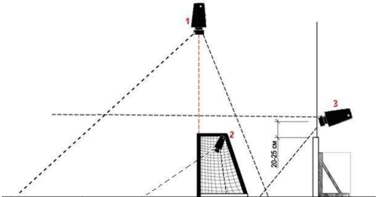
3.2 Locations of cameras above the goal net and behind the goal net (side view)
